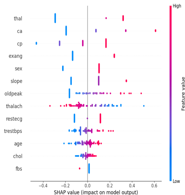
Figure 8: SHAP Summary Plot for LR
