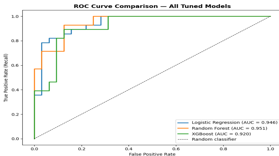
Figure 11: ROC Curve Comparison of Tuned Logistic Regression, Random Forest, and XGBoost Models.
