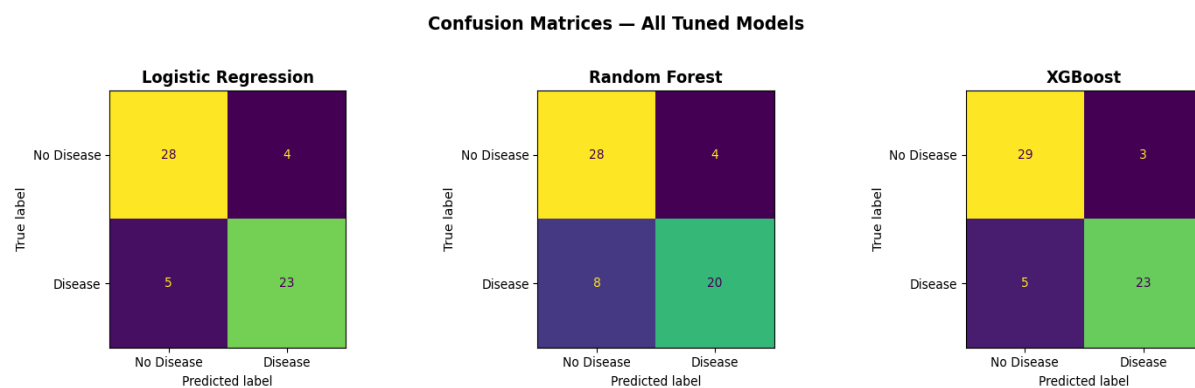
Figure 12: Confusion Matrices
